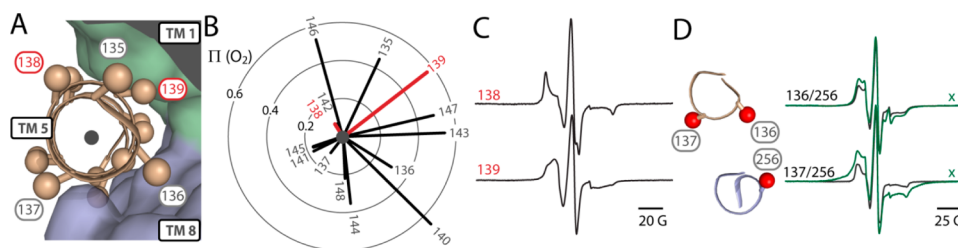
Figure 2. Orientation of TM 5 conflicts with the crystal structure. (A) Positions on TM 5 where accessibility and mobility were probed are highlighted as spheres. TM 5 (ribbon) is shown against a surface representation of the rest of EmrD to depict tertiary interactions. (B) Vectors indicate O_2 accessibility ( \Pi ) throughout TM 5. The orientation of the plot matches the orientation of TM 5 in panel A, and vectors were drawn from the center of the helix (black dot) through the \beta carbon of the side chain. Representative positions 138 and 139 are highlighted in red. (C) CW-EPR spectra of positions 138 and 139 (red in panels A and B). (D) Cross-section of the TM 5–TM 8 interface indicates the predicted orientation of residues 136, 137, and 256. CW-EPR spectra of double Cys mutants (green) show strong dipolar coupling (spectral broadening) between labels at 137 and 256 relative to the sum of the spectra from single mutants (black). The y-axes of the spectra from double mutants were scaled as indicated.
