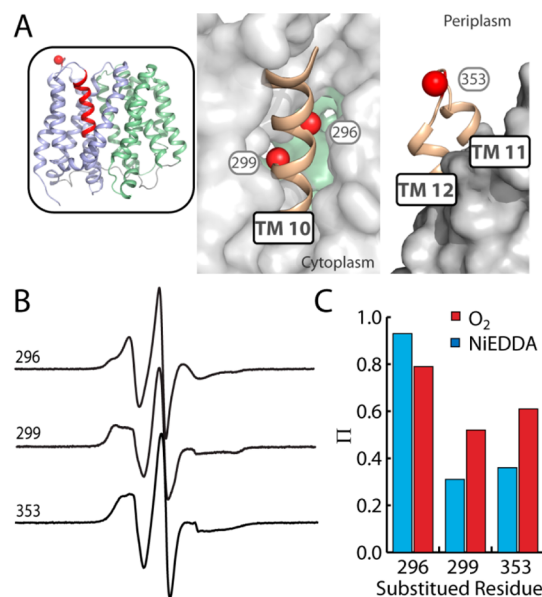
Figure 3. Topology of TMs 10–12 deviates from the crystal structure. (A) Positions on TM 10 and the periplasmic loop between TMs 11 and 12 where mobility and accessibility were probed are highlighted as spheres. Regions of interest (ribbon) are shown against a surface representation of the rest of EmrD to depict tertiary interactions and proximity of TM 10 to the central cavity. (B) CW-EPR spectra showing the mobility of spin labels at the three positions. (C) The accessibility ( \Pi ) of spin labels to O 2 (red) or NiEDDA (blue).
