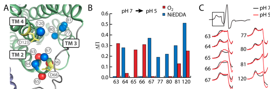
Figure 4. Low pH opens a cytoplasmic cleft. (A) Positions in TMs 2–4 where significant changes in Ni-EDDA (blue) or O 2 (red) accessibility and/or mobility are represented as spheres on the structural model of EmrD. Conserved acidic residues are highlighted in yellow. (B) Change in NiEDDA (blue) or O 2 (red) accessibility from pH 7 to pH 5. (C) CW-EPR spectra indicating increased mobility at pH 5 (red) versus pH 7 (black). Only the low field resonance line is shown for clarity.
