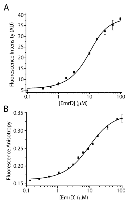
Figure 7. Binding of Hoechst and doxorubicin. Increasing concentrations of EmrD were incubated with 5 \mu\text{M} substrate in GF buffer as described in Experimental Procedures. Binding was inferred from an increase in the fluorescence intensity of Hoechst (A) or the anisotropy of doxorubicin (B). Solid lines are nonlinear least-squares fits with a K_D values of 3 \mu\text{M} for Hoechst (A) and 7 \mu\text{M} for doxorubicin (B).
