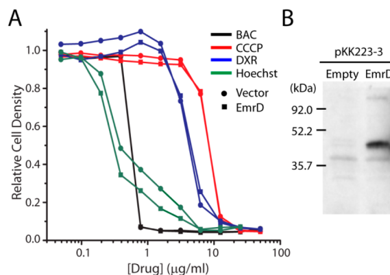
Figure 9. EmrD expression did not confer multidrug resistance. (A) Drug sensitive E. coli expressing WT EmrD (squares) or harboring empty pKK223-3 vector (circles) were cultured in wells containing 50% LB, 0.1 mg/mL ampicillin, and 0–50 \mu g/mL benzalkonium chloride (BAC; black), CCCP (red), doxorubicin (DXR; blue), or Hoechst 33342 (green). Optical density is plotted relative to the growth of the drug-free culture. (B) Anti-His immunoblot of inside-out membrane vesicles isolated from drug sensitive E. coli expressing WT EmrD with an N-terminal His-10 tag or harboring the empty pKK223-3 vector.
